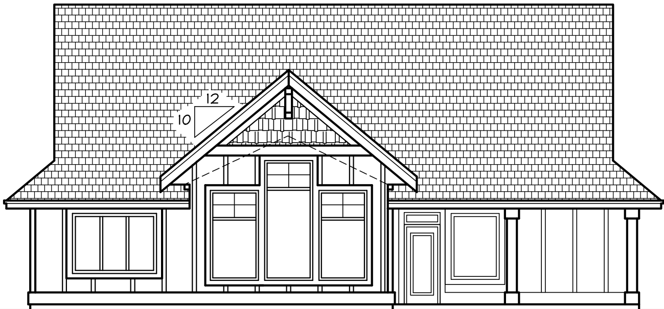
REAR ELEVATION
